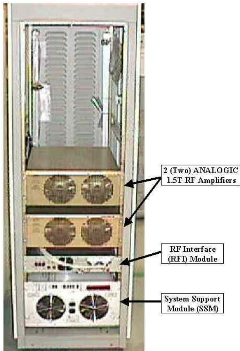
1.5T SRF CABINET ILLUSTRATION 1-1
