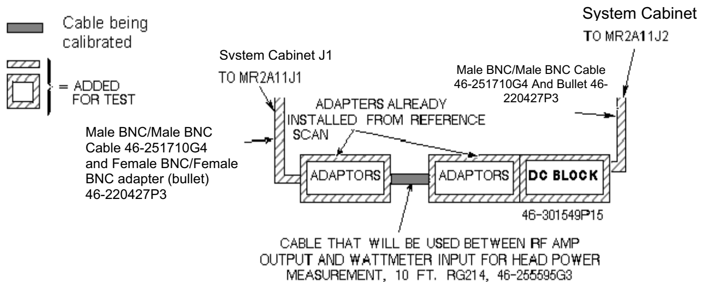
CONNECTIONS FOR DUMMY LOAD + CABLES SCAN ILLUSTRATION F4-1
