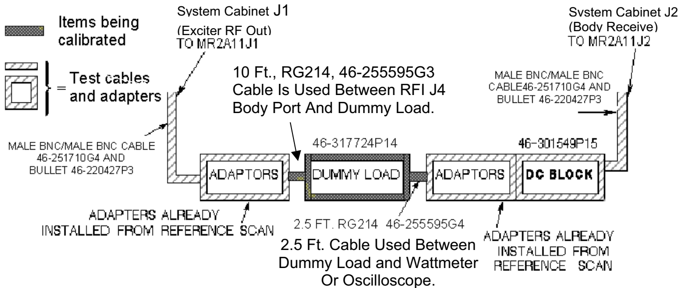
CONNECTIONS FOR DUMMY LOAD + CABLES SCAN ILLUSTRATION F4-1
